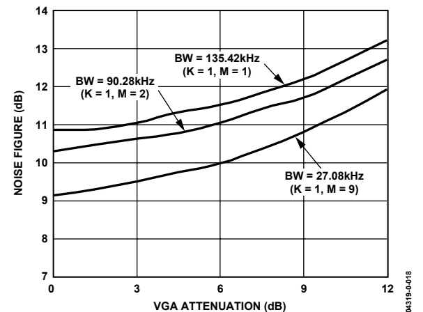
Figure 19. Noise Figure vs. VGA Attenuation ( f_{CLK} = 26 MSPS)
